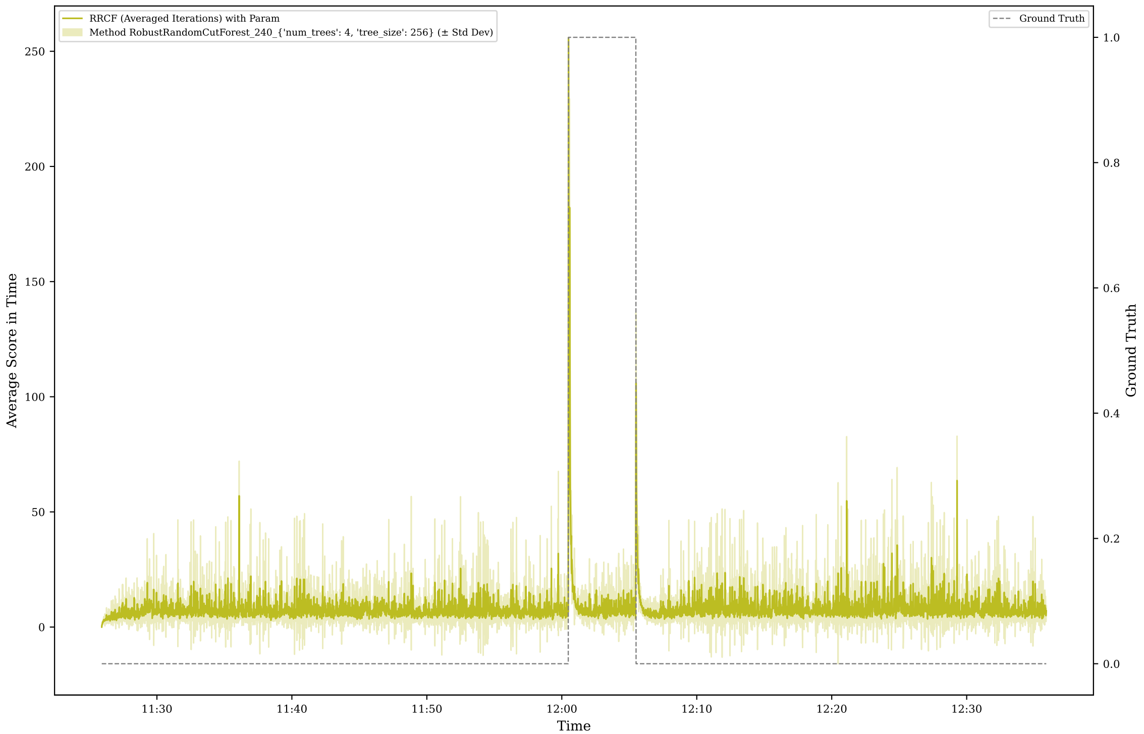
Method RRCF Score for Scenario A5
